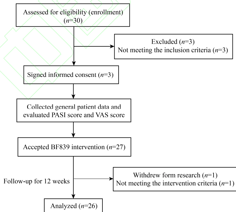
Fig. 1 Experimental flowchart.
